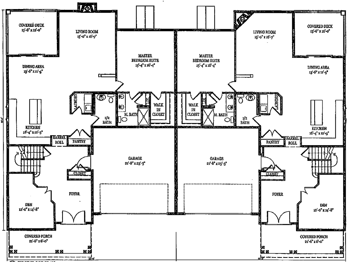
○ FIRST FLOOR PLAN N.T.S. 1811 SQUARE FOOTAGE
